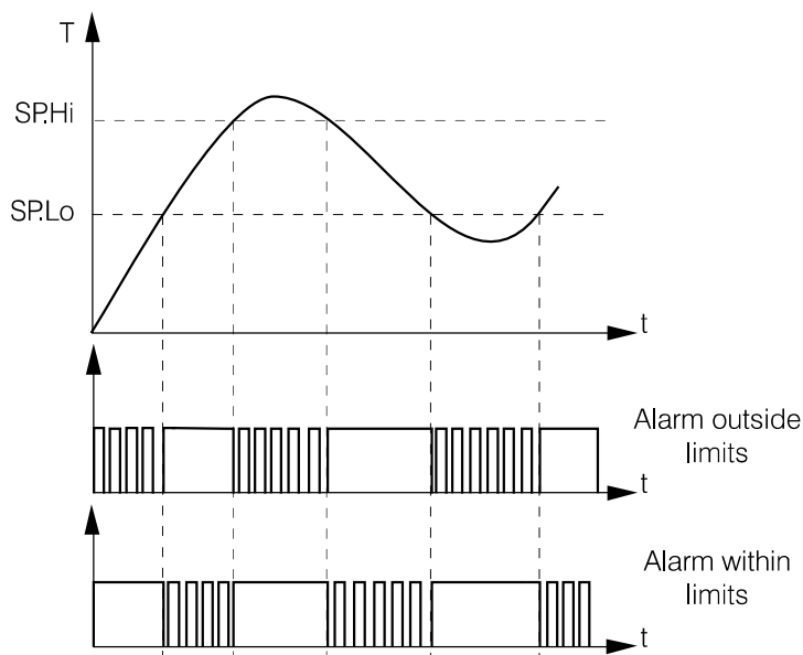
Fig 6.2 Alarm function
