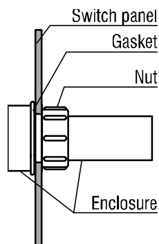
Fig. 5.1 Mounting
