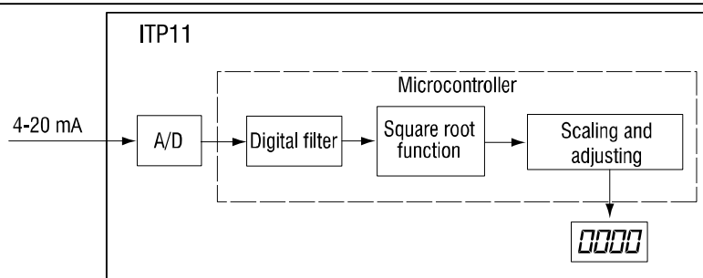
Fig. 4.1 Block diagram
