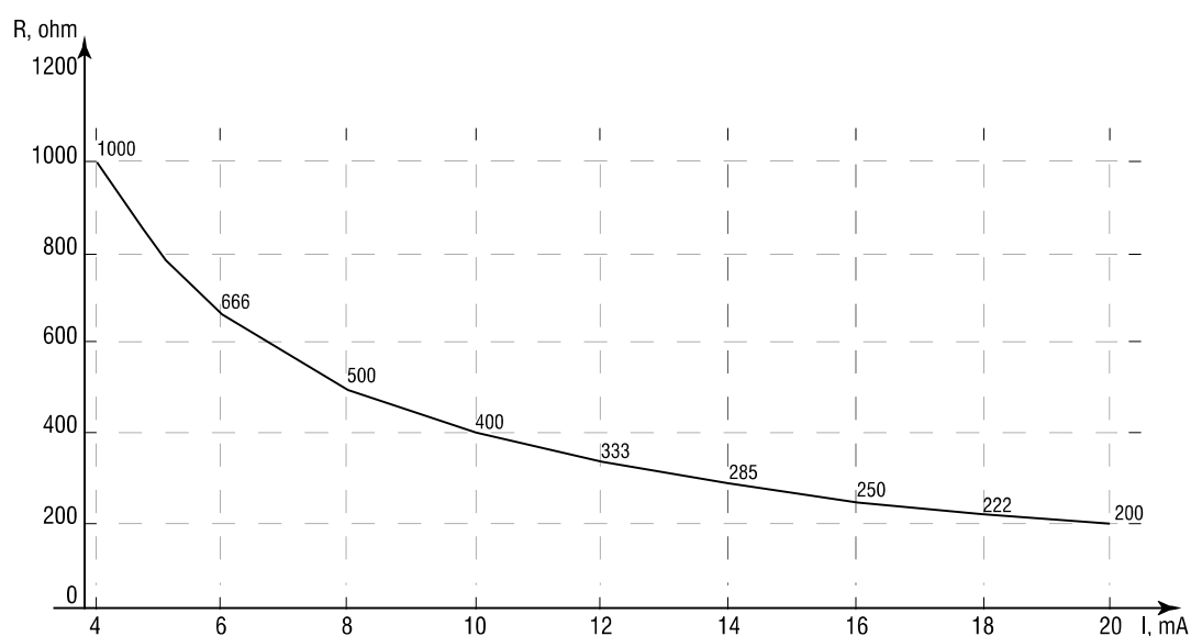
Fig. 2.1 Input resistance *
